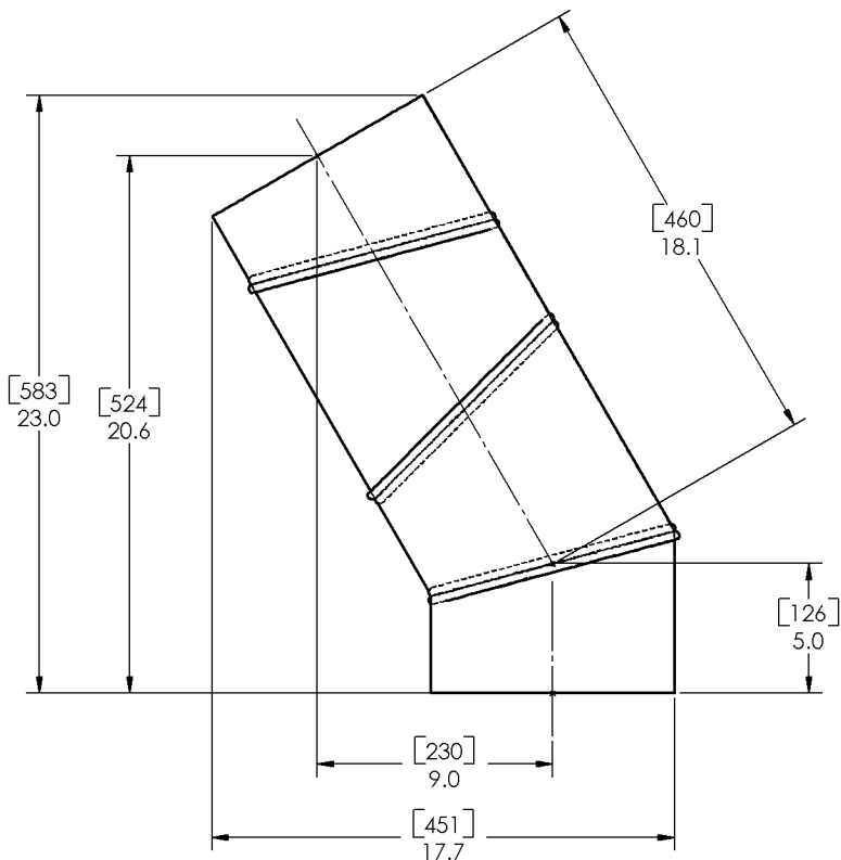
30° ANGLE SCALE 1:1
