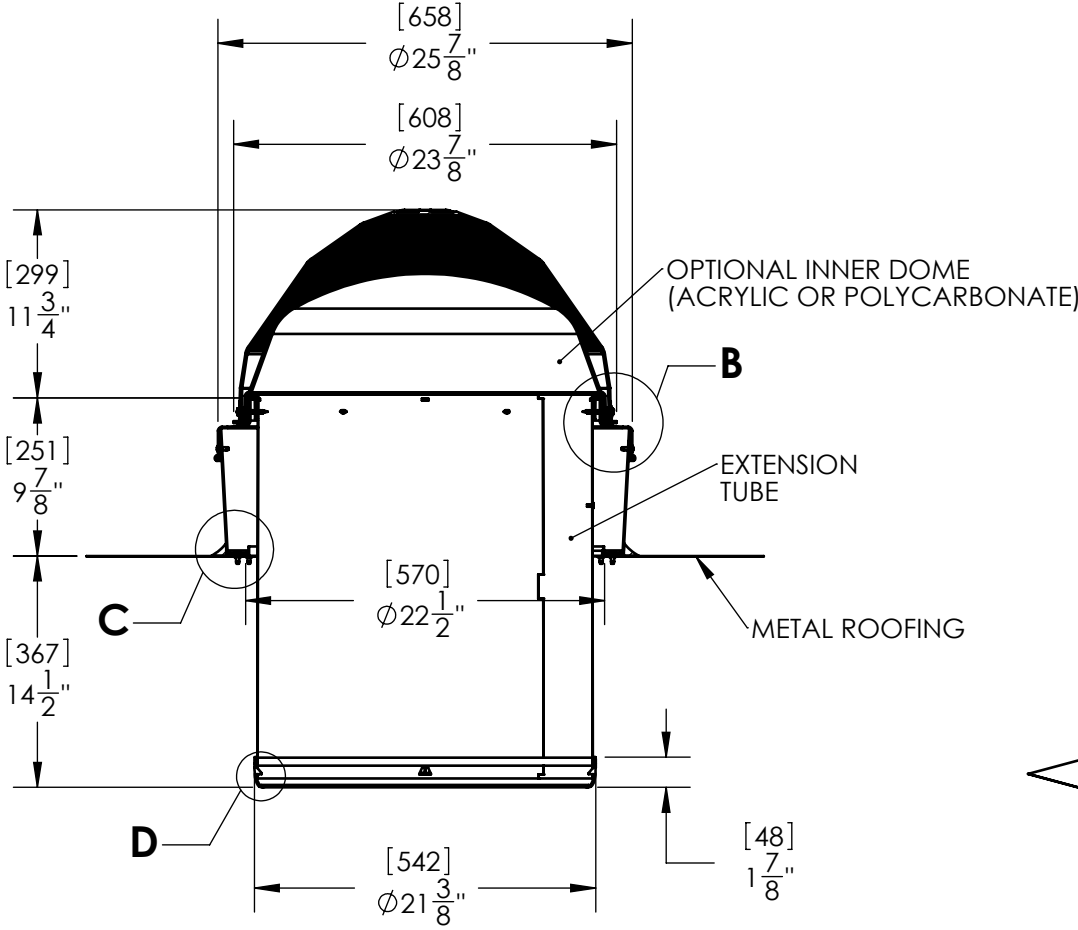
FULL SECTION
