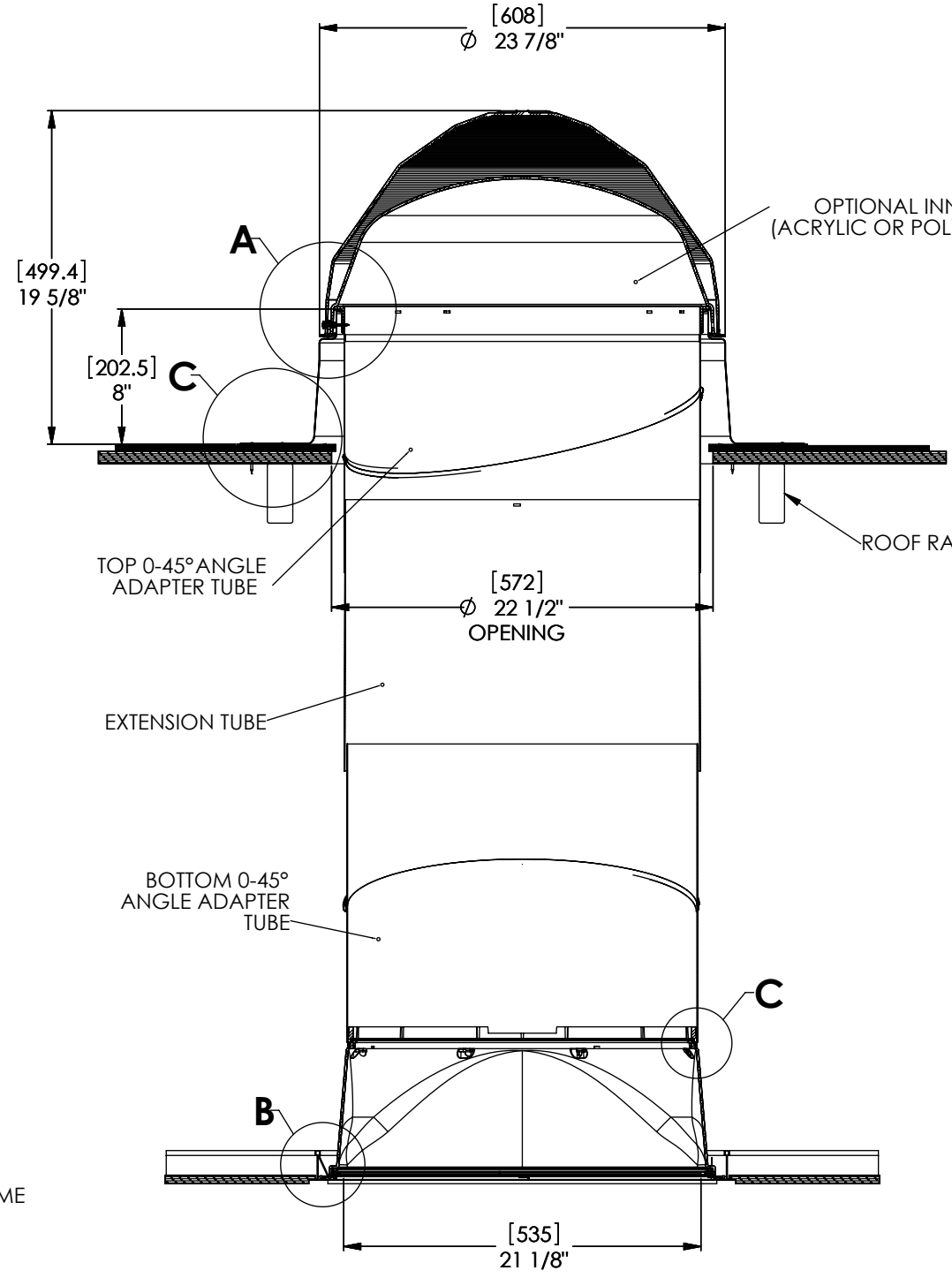
FULL SECTION SCALE 1:1
